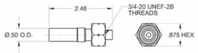
Chatleff Adapter Assembly
