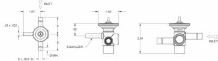
Non-Adjustable - ODF Connections with 1/4 ODF Equalizer Shown
